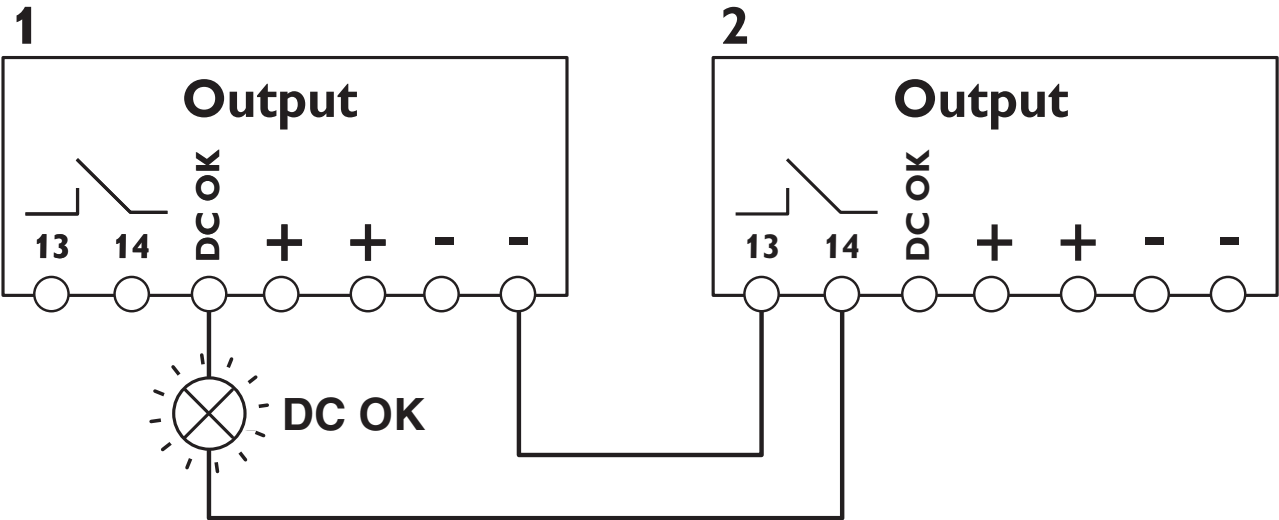
Circuit diagram
