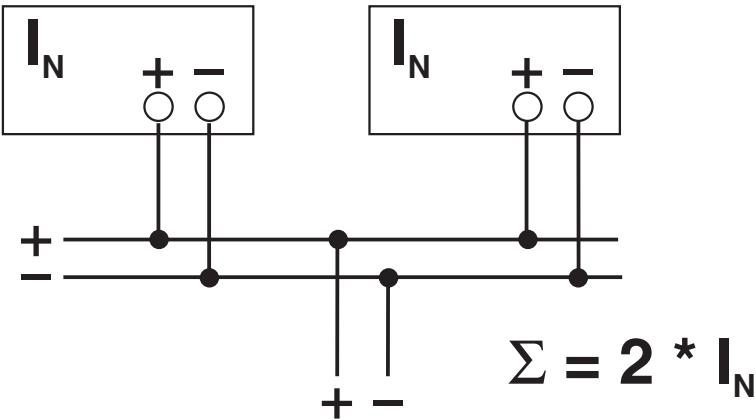
Circuit diagram
